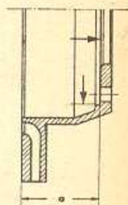
Rear wheel brake disc
