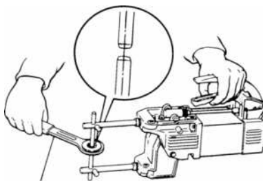
Tip Cutter
