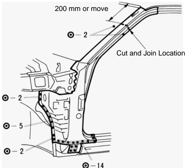
Front Body Pillar Lower Gusset
