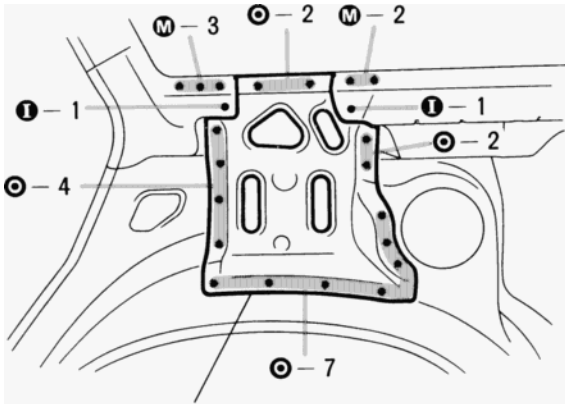
Roof Side Inner to Wheel Housing Brace
