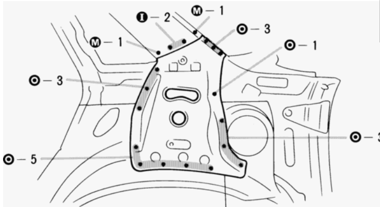
Roof Side Outer Panel
